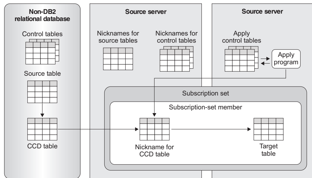
Figure 7. Replicating data from non-DB2 sources to DB2 UDB targets.. Triggers populate a staging table called a consistent-change-data (CCD) table with records of changes made to a source table. The Apply program reads the CCD table through that table's nickname on the DB2 II federated database. The Apply program then makes the appropriate changes to the target table.
