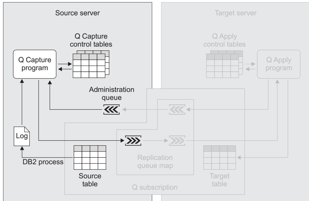
Figure 12. Capturing data in Q replication. The Q Capture program reads the DB2 recovery log for changes made to your sources and converts committed transactional data to messages, which it puts on a send queue. The Q Capture program continuously updates its control tables with information that you can use to monitor its progress.
