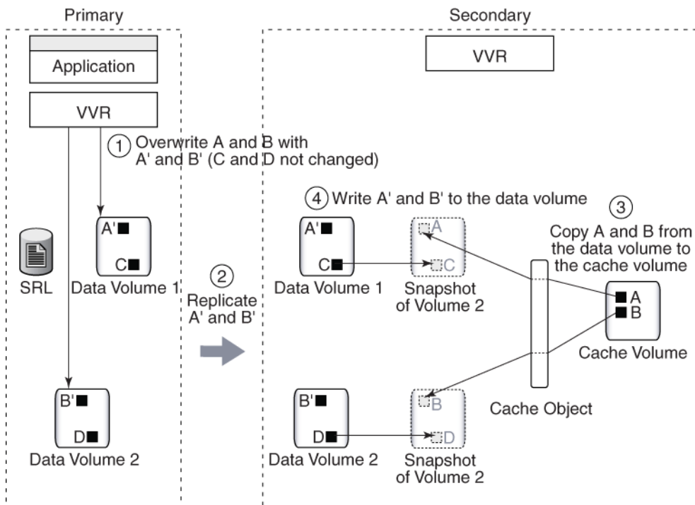
Example 2—How VVR Writes to the Instant Space-Optimized Snapshots
