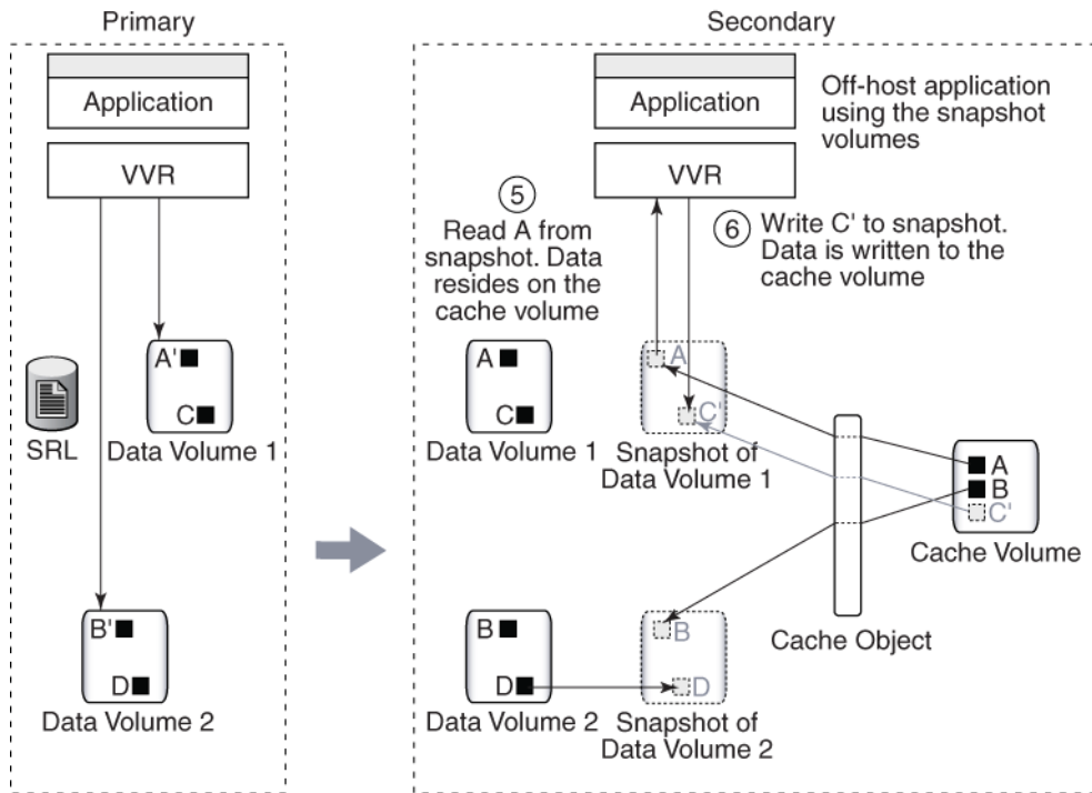
Example 3—How VVR Reads the Changed Block from the Cache Object
