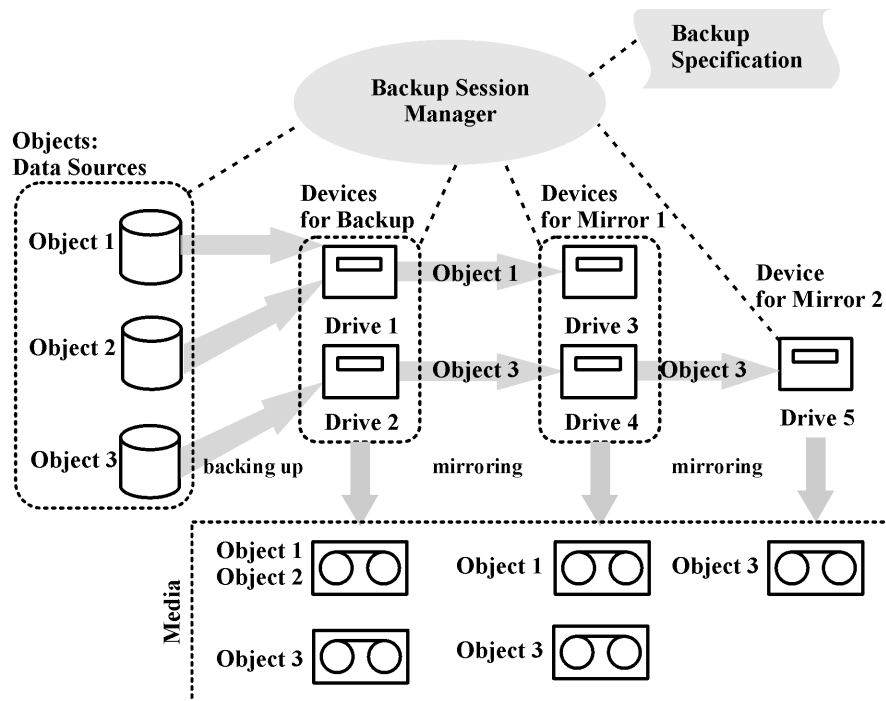
Figure 2-17 Object Mirroring
