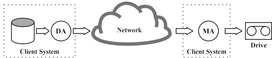
Figure 1-6 Backup Session
