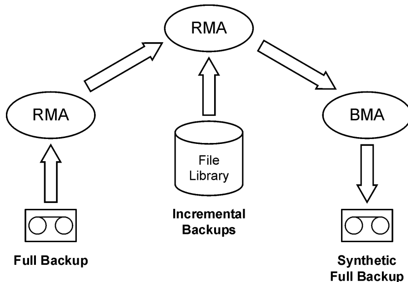
Figure 11-1 Synthetic Backup
