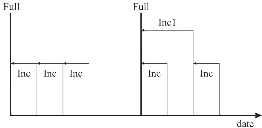
Figure 2-5 Differential Backups
