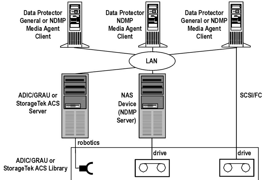
Figure 3-15 Sharing an ADIC/GRAU or StorageTek ACS Library
