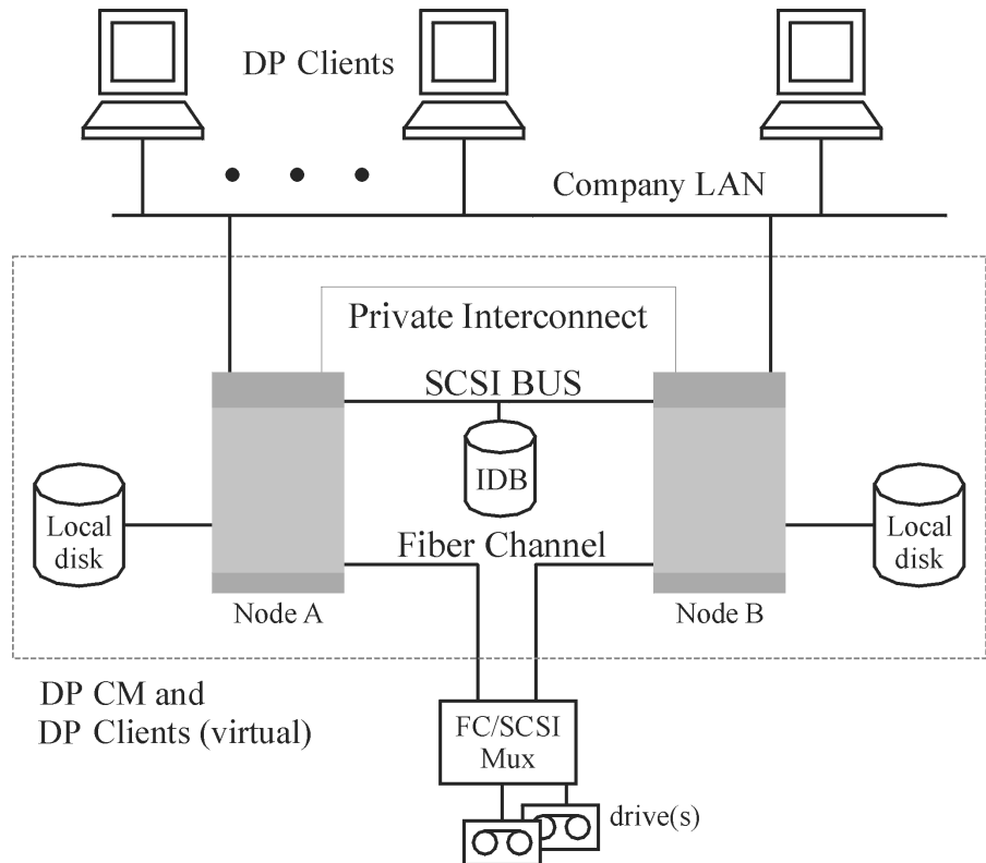
Figure 2-4 Cell Manager Installed in the Cluster, Devices Connected to Cluster Nodes
