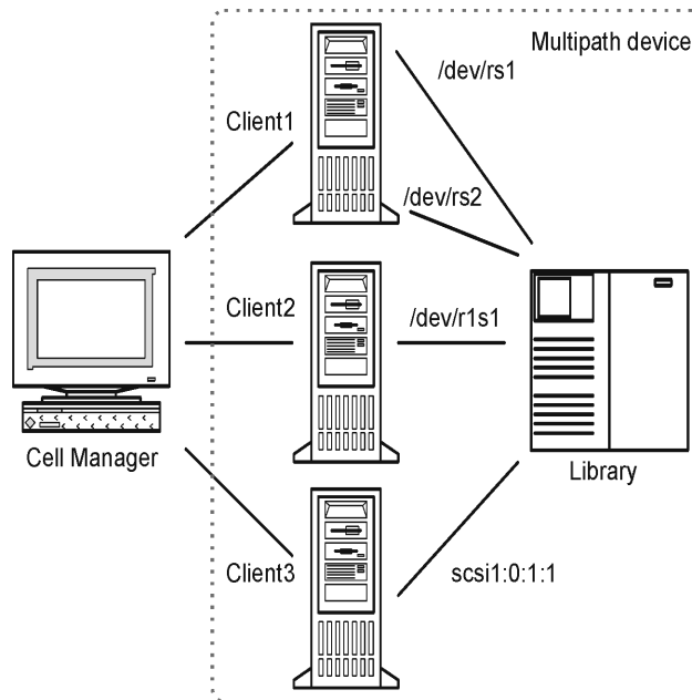
Figure 3-18 Example Multipath Configuration
