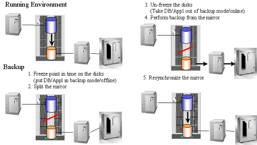
Figure 12-1 Split Mirror Backup Concept
