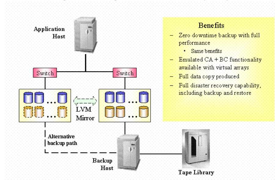
Figure 13-6 LVM Mirroring - HP StorageWorks Virtual Array Only
