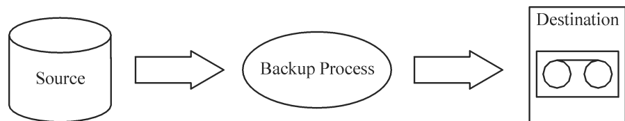
Figure 1-1 Backup Process
