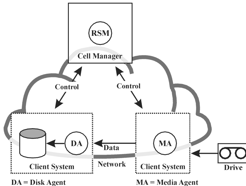
Figure 7-3 Restore Session Information Flow
