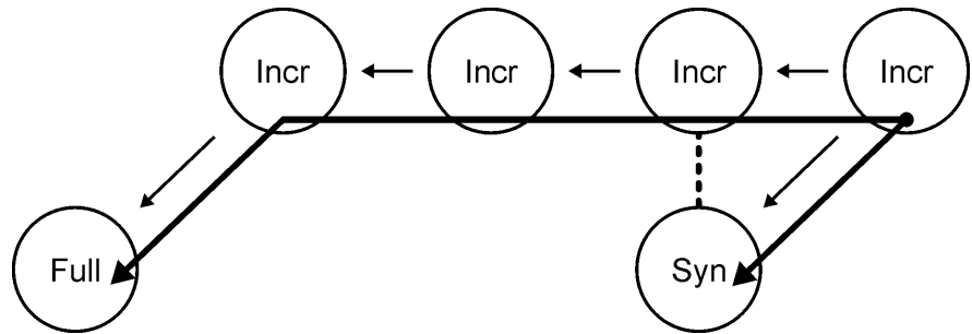
Figure 11-4 Synthetic Backup
