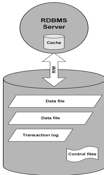
Figure 8-1 Relational Database
