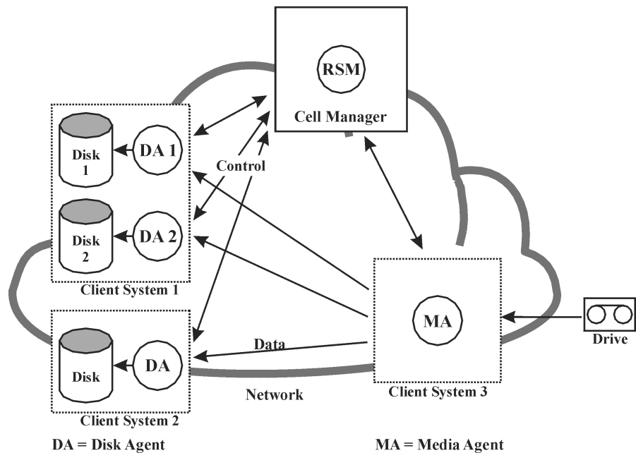
Figure 7-4 Parallel Restore Session Flow
