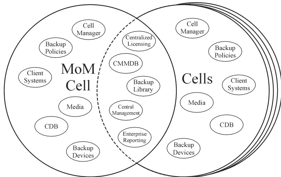
Figure 1-10 Manager-of-Managers Environment
