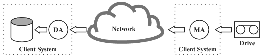
Figure 1-7 Restore Session
