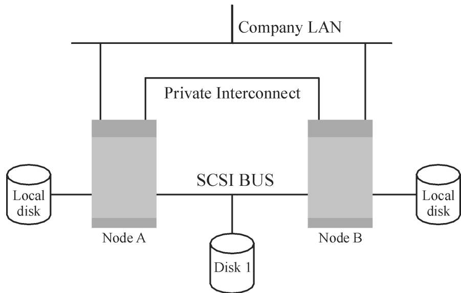
Figure 2-1 Typical Cluster
