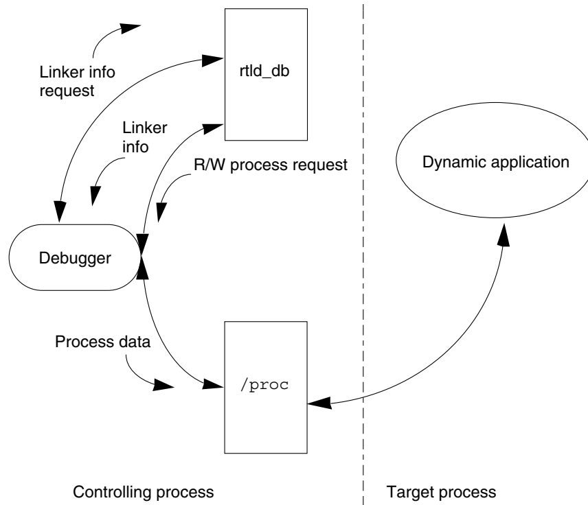
FIGURE 6-1 rtld-debugger Information Flow
