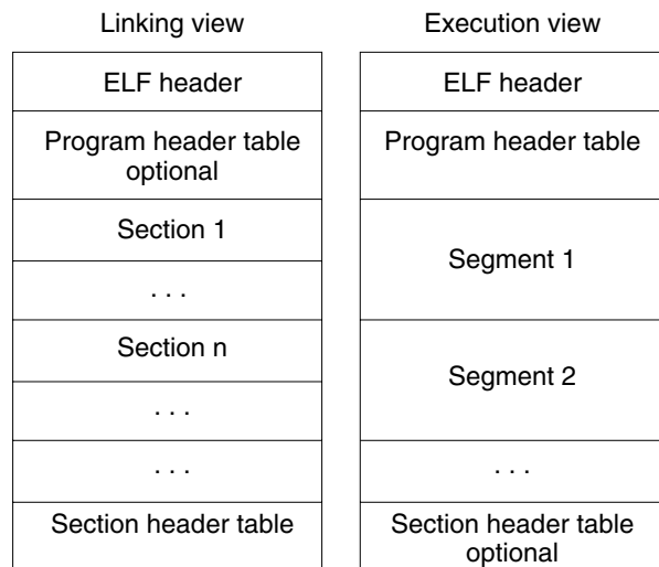
FIGURE 7-1 Object File Format
