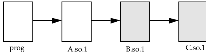
FIGURE 3-1 A Single dlopen() Request
