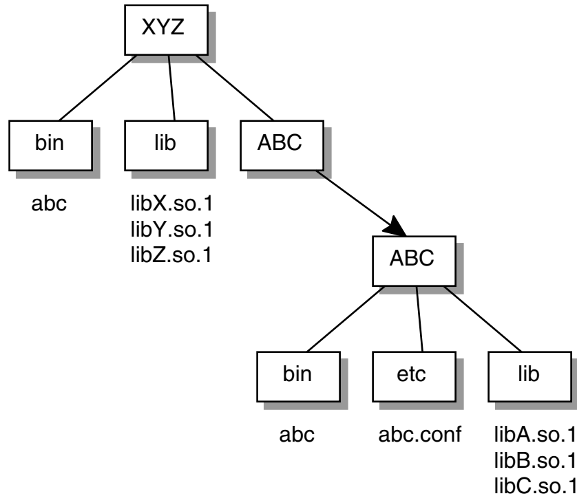
FIGURE C-2 Unbundled Co-dependencies
