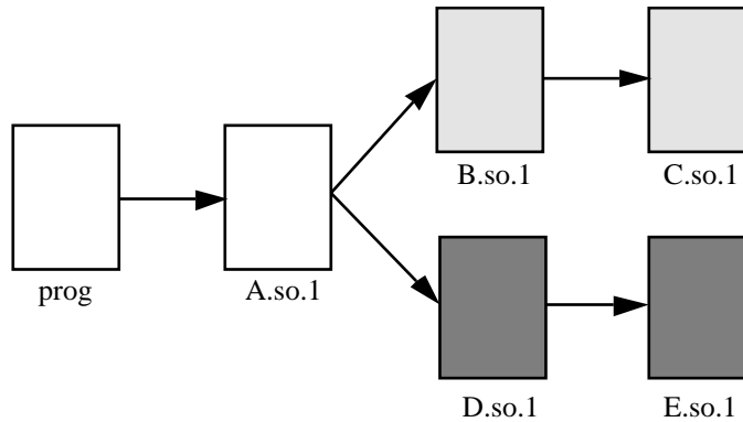
FIGURE 3-2 Multiple dlopen() Requests
