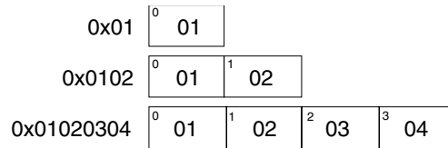
FIGURE 7-3 Data Encoding ELFDATA2MSB
