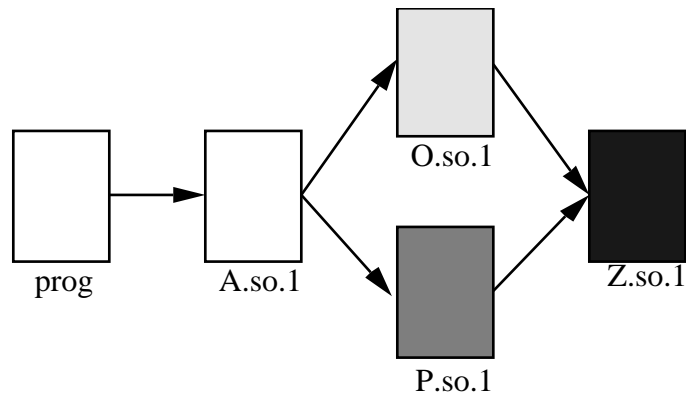
FIGURE 3-3 Multiple dlopen() Requests With A Common Dependency
