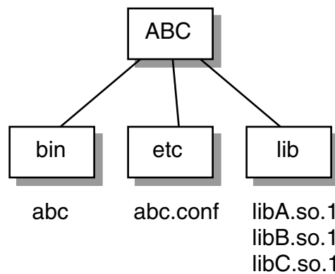
FIGURE C-1 Unbundled Dependencies
