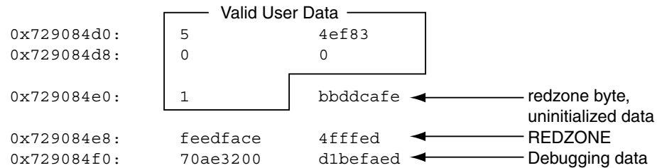
FIGURE 8-2 Sample kmem_alloc(9F) Buffer
