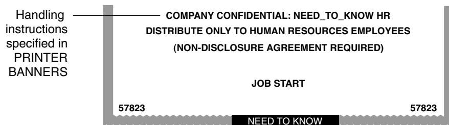
FIGURE 4-5 Commercial Use of PRINTER BANNERS on Banner Page
