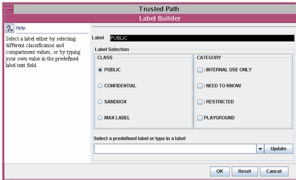
FIGURE 5-1 Column Headers on Label Builder
