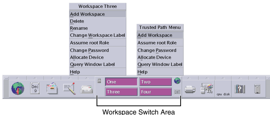
FIGURE 1-9 Workspace Switch Area
