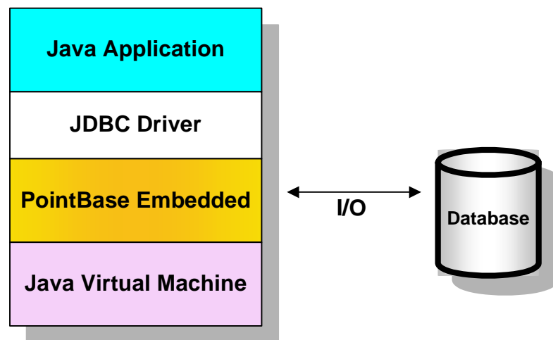
Figure 1.2 Using PointBase Embedded
