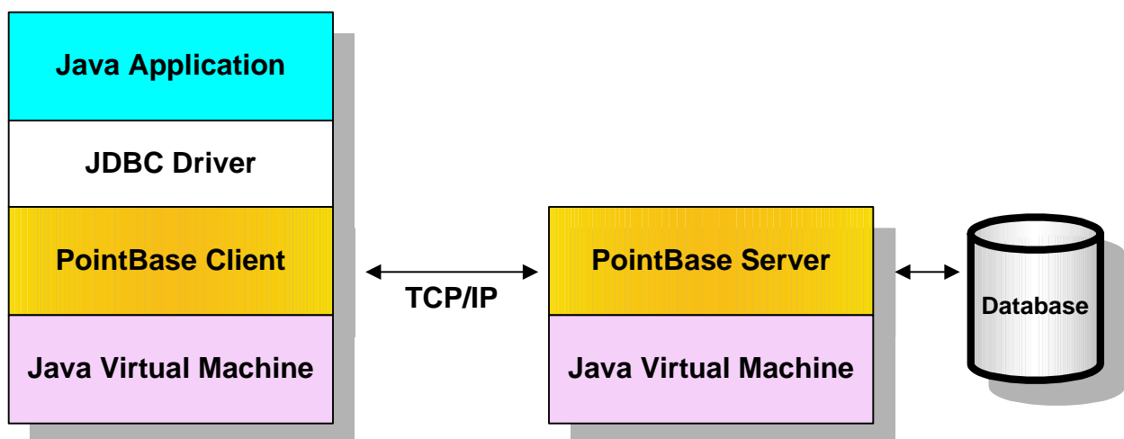
Figure 1.3 Using PointBase Server Option
