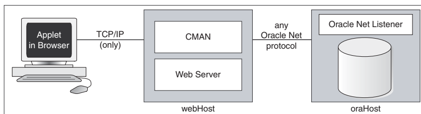
Figure 4-1 Applet, Connection Manager, and Database Relationship
