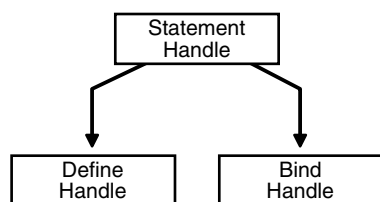
Figure 2-3 Statement Handles
