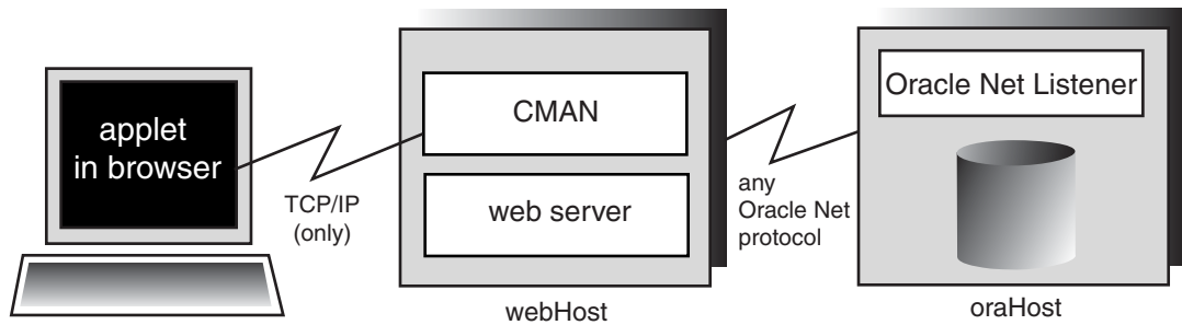
Figure 24-1 Applet, Connection Manager, and Database Relationship
