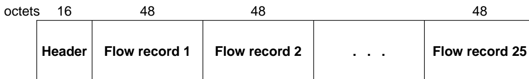
Figure 36: Format of NetFlow export datagram
