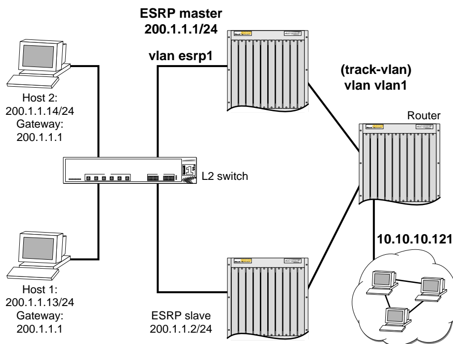
Figure 45: ESRP tracking
