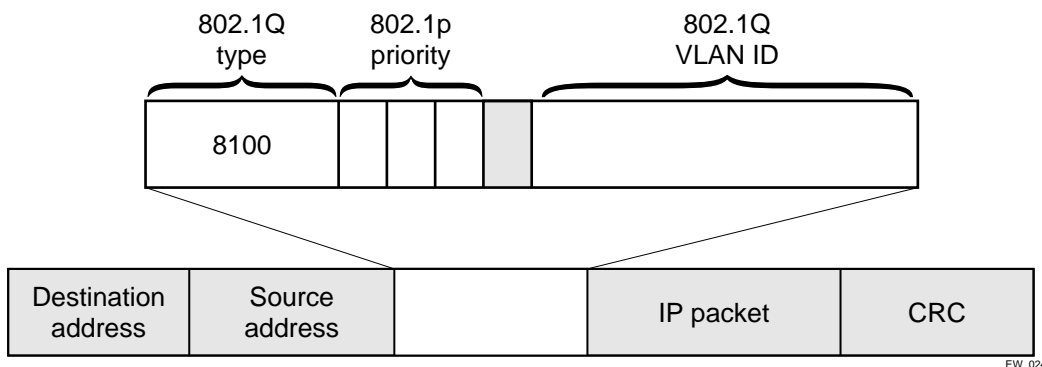
Figure 11: Ethernet packet encapsulation
