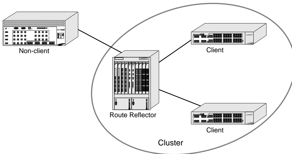
Figure 67: Route reflectors
