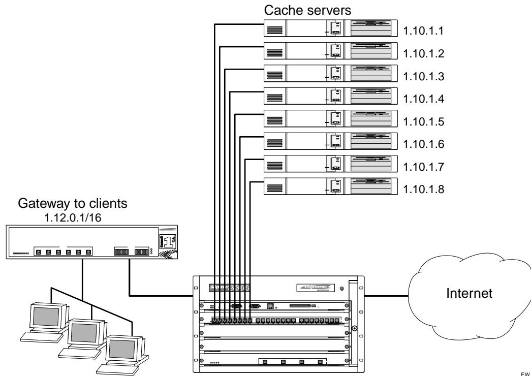
Figure 31: Web cache redirection example
