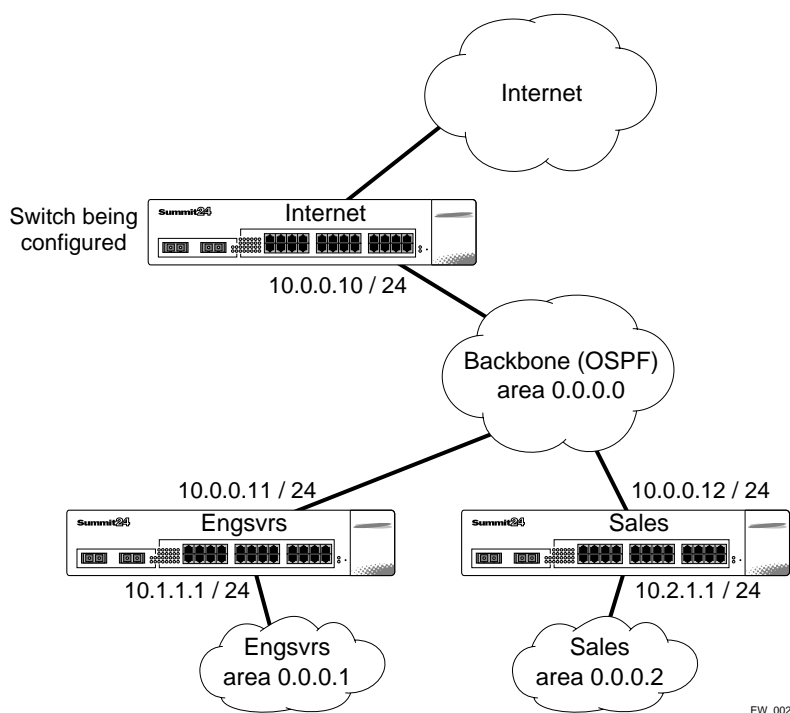
Figure 20: OSPF access policy example
