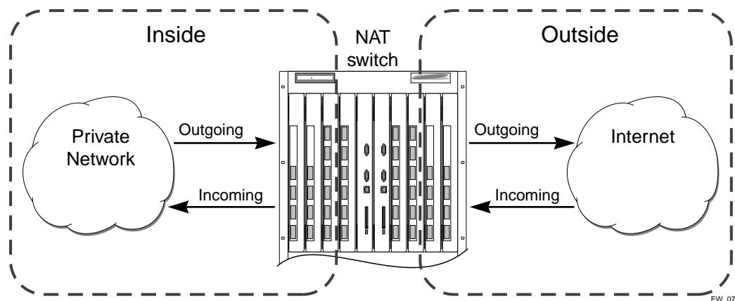
Figure 22: NAT Overview
