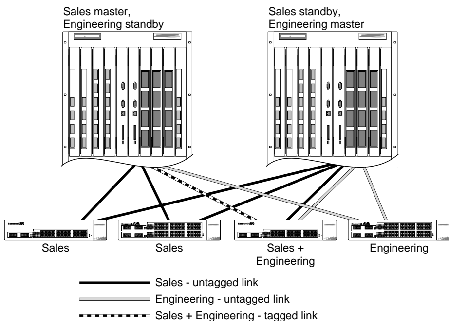
Figure 55: ESRP example using layer 2 redundancy
