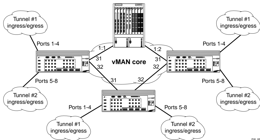
Figure 9: VMAN example
