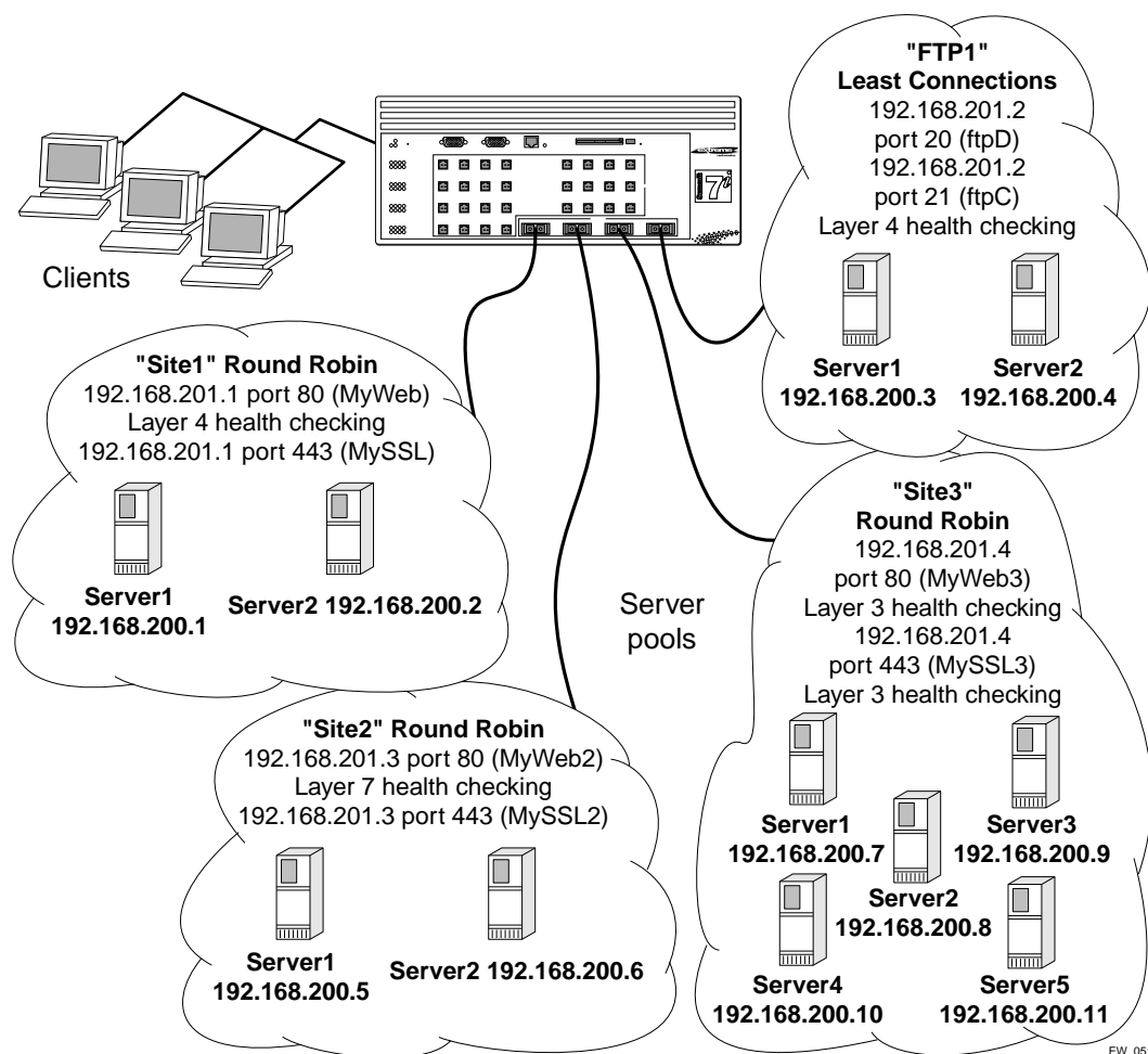
Figure 28: Advanced SLB configuration
