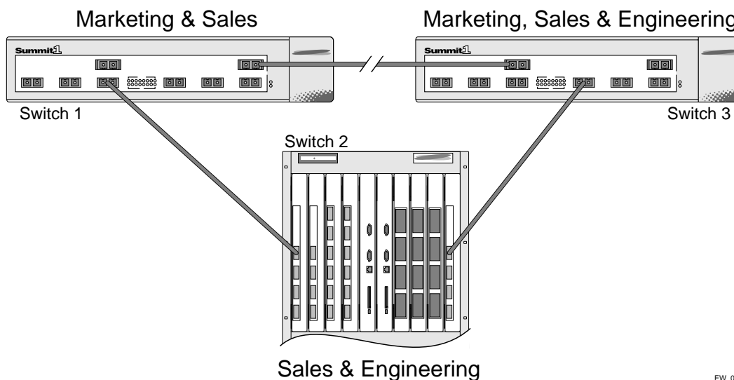
Figure 39: Tag-based STP configuration
