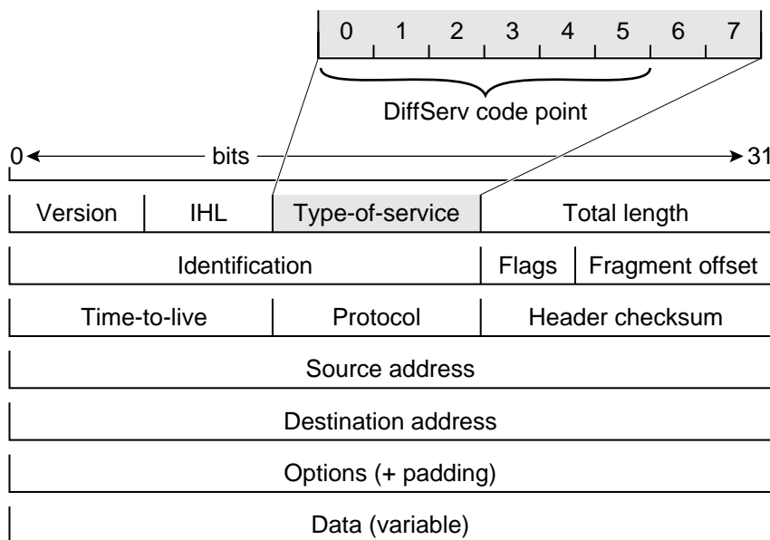
Figure 12: IP packet header encapsulation
