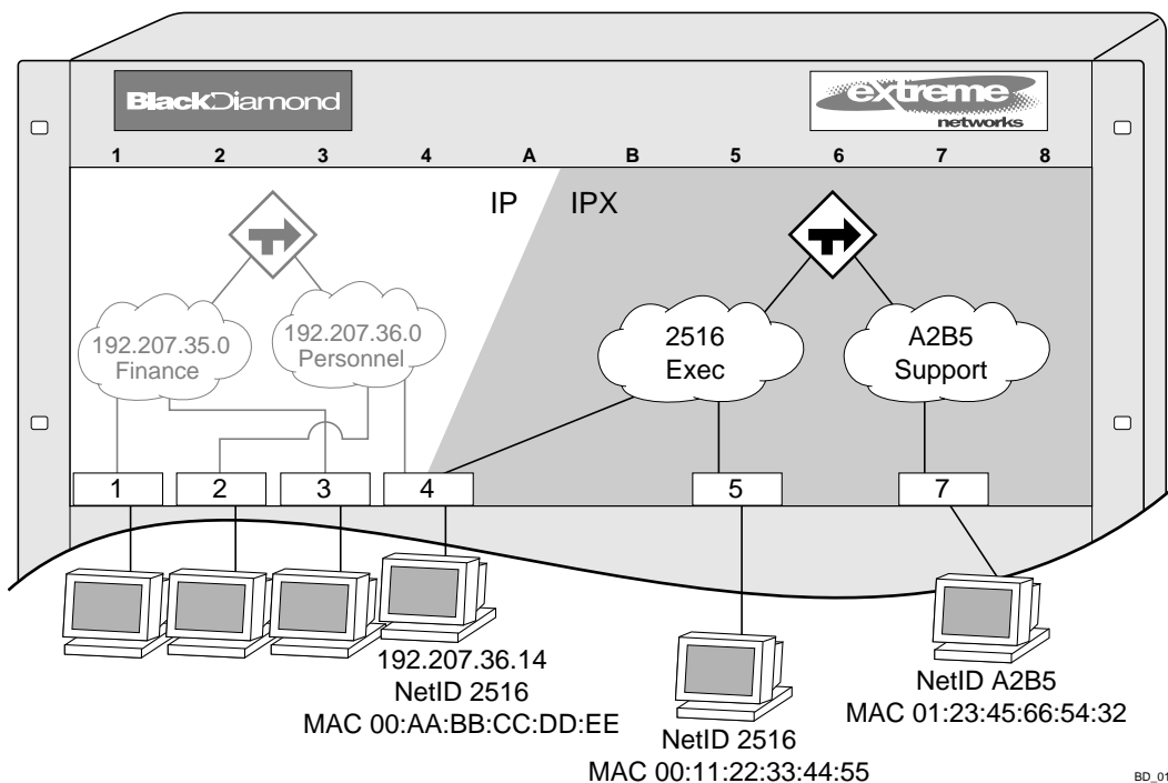
Figure 71: IPX VLAN configuration
