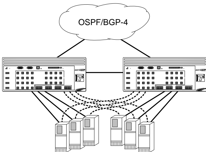
Figure 51: ESRP host attach
