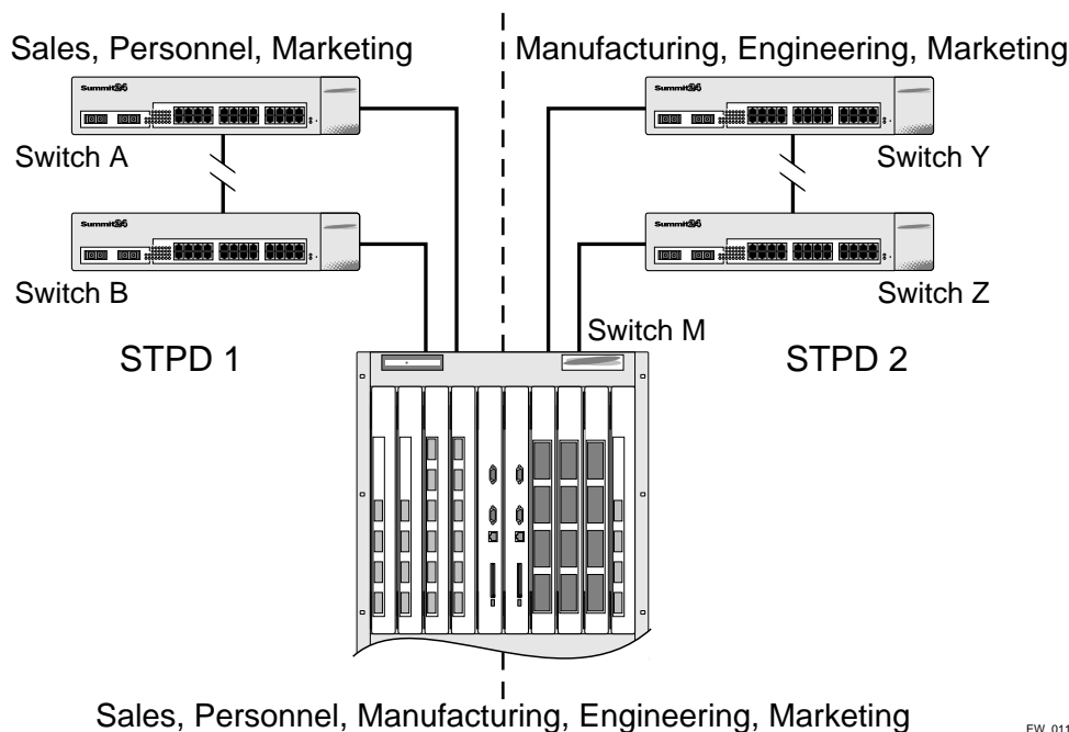
Figure 38: Multiple Spanning Tree Domains
