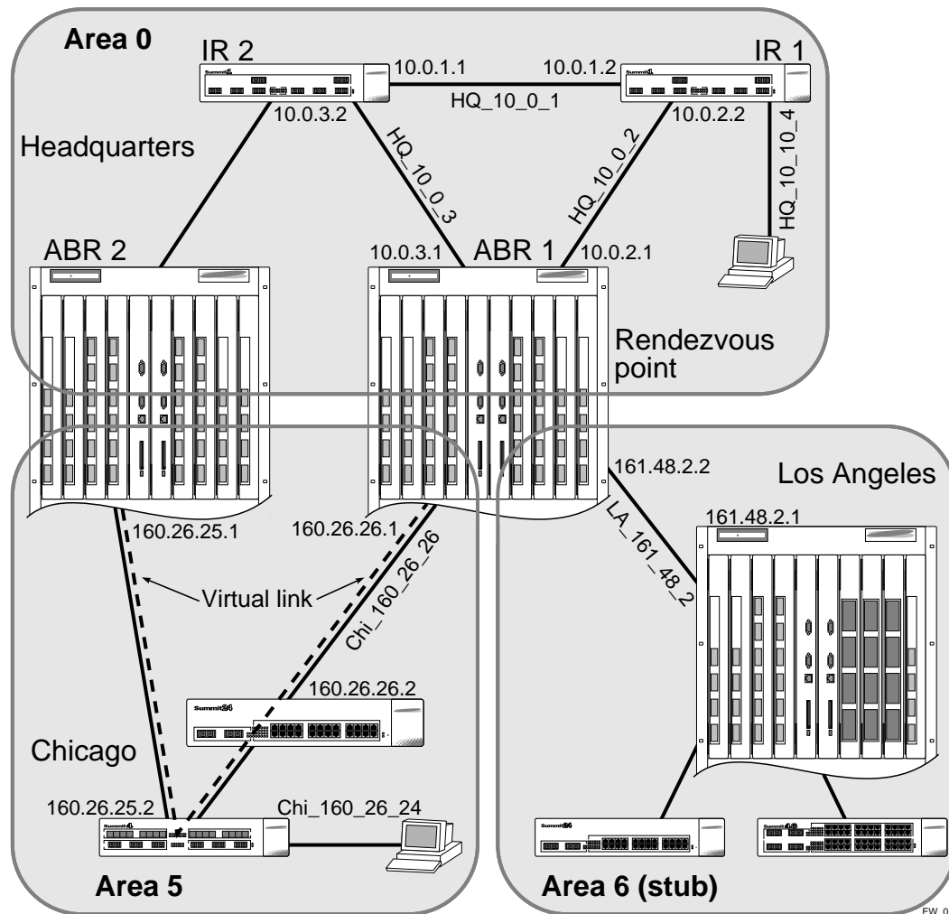
Figure 70: IP multicast routing using PIM-SM configuration example
