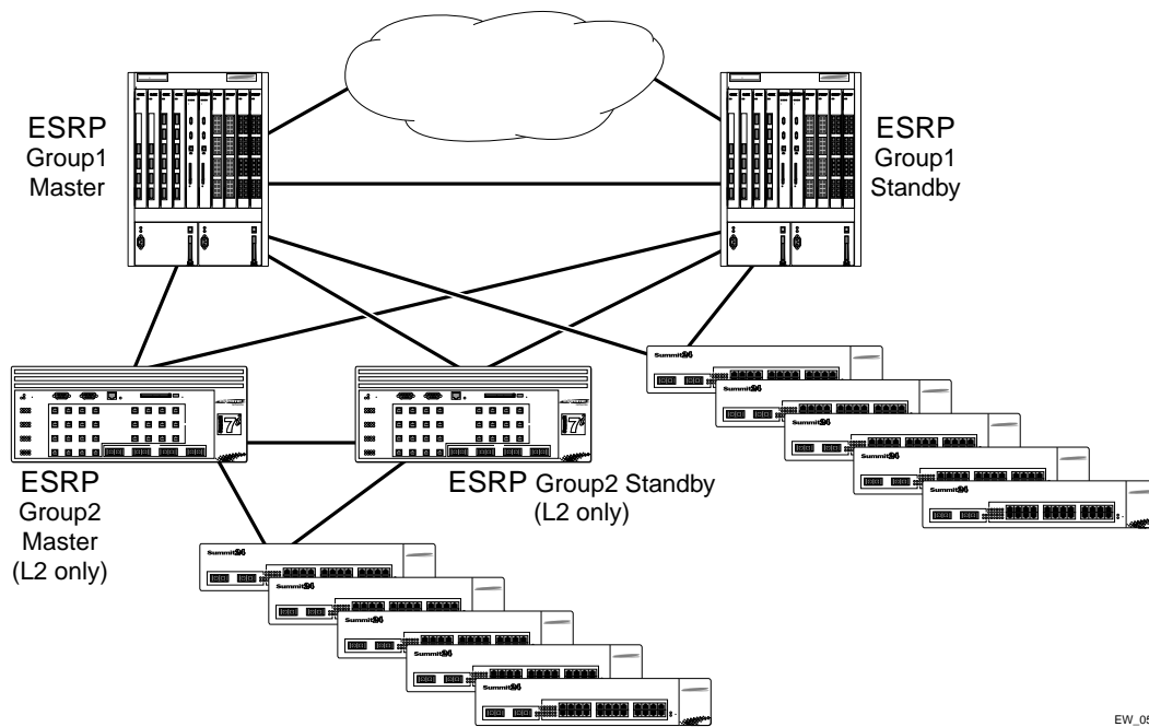
Figure 53: ESRP groups
