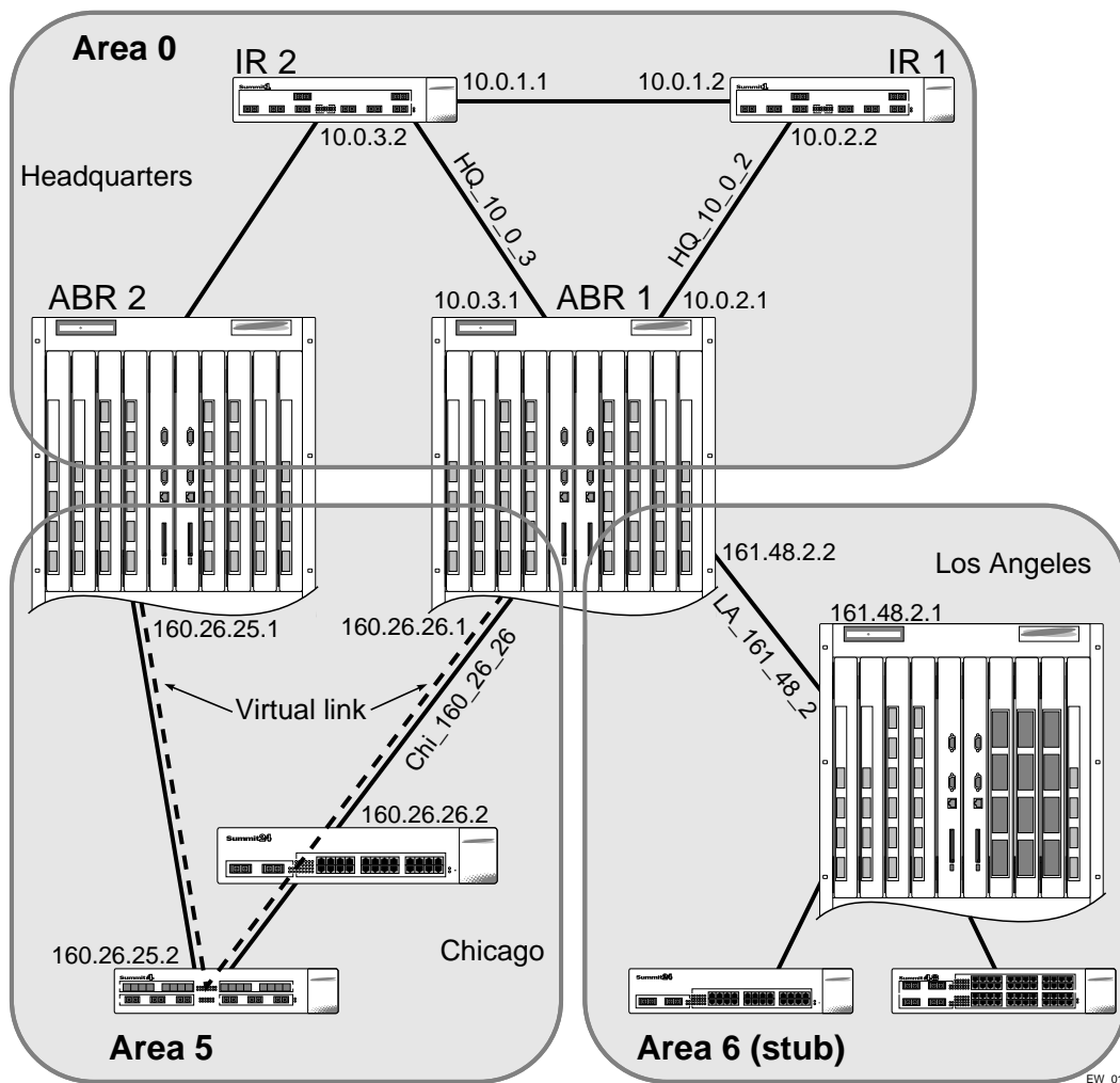
Figure 66: OSPF configuration example
