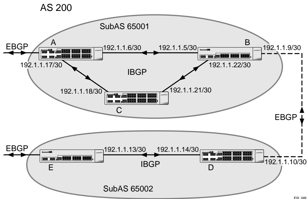
Figure 68: Routing confederation
