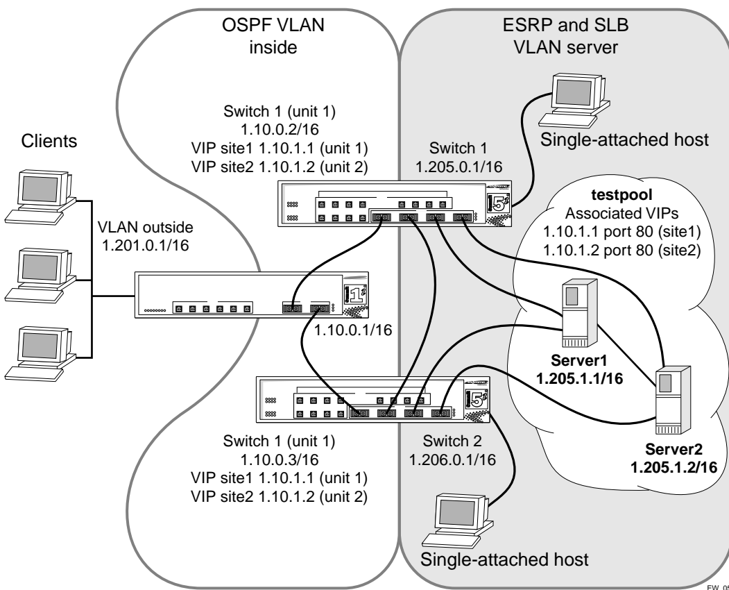
Figure 29: SLB using ESRP and dual-homed servers
