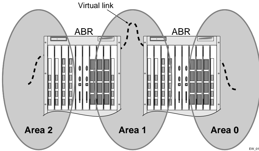
Figure 62: Virtual link using Area 1 as a transit area
