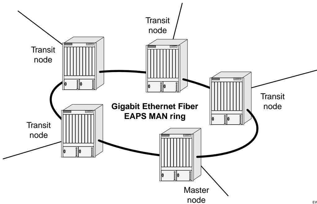
Figure 32: Gigabit Ethernet fiber EAPS MAN ring
