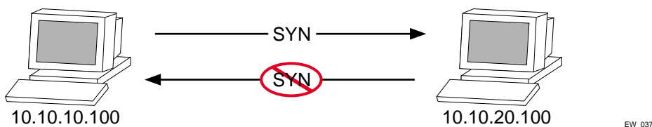
Figure 17: Permit-established access list filters out SYN packet to destination
