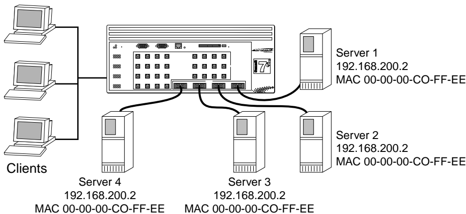
Figure 27: GoGo mode
