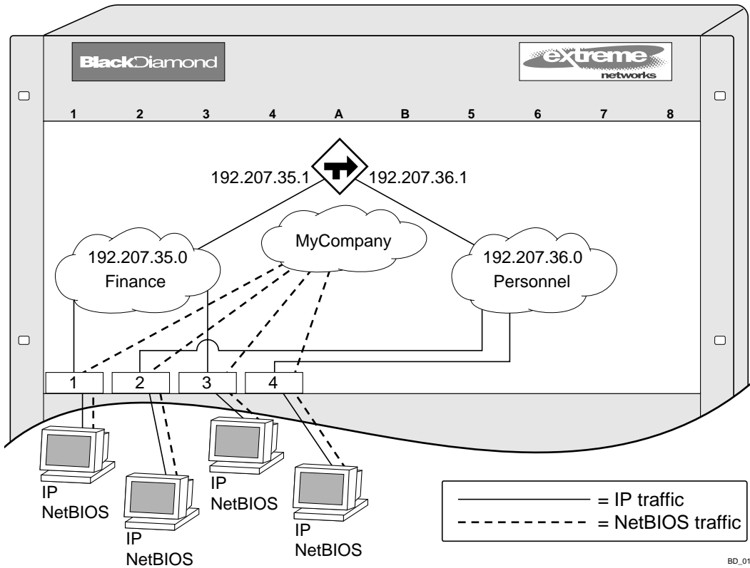
Figure 60: Unicast routing configuration example
