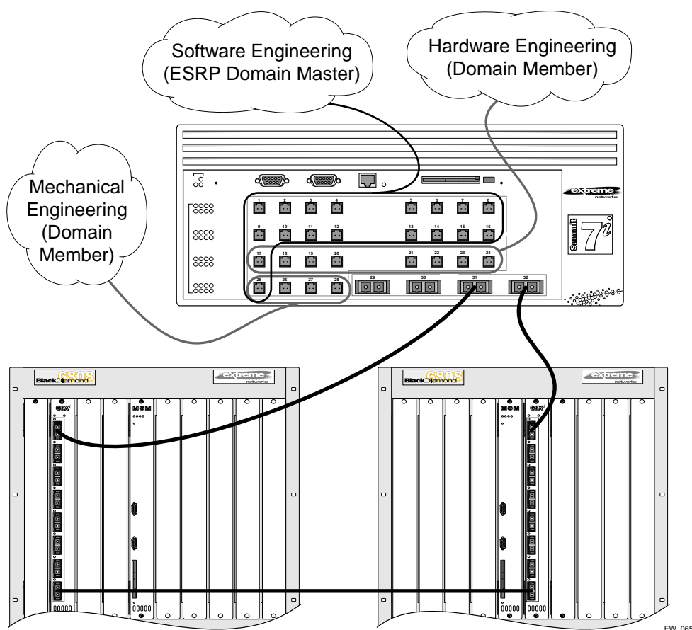
Figure 52: ESRP domains
