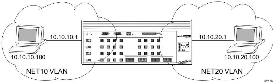
Figure 13: Permit-established access list example topology
