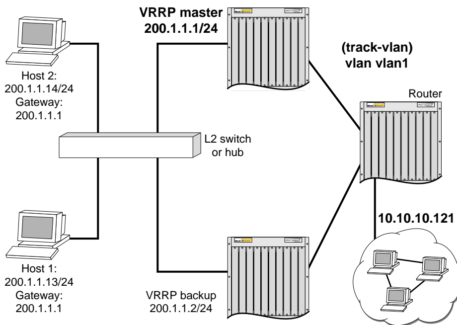
Figure 56: VRRP tracking
