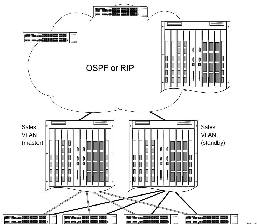
Figure 54: ESRP example using layer 2 and layer 3 redundancy
