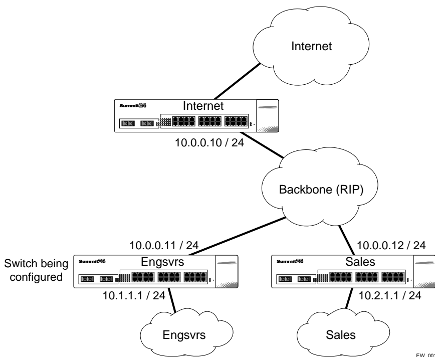
Figure 19: RIP access policy example
