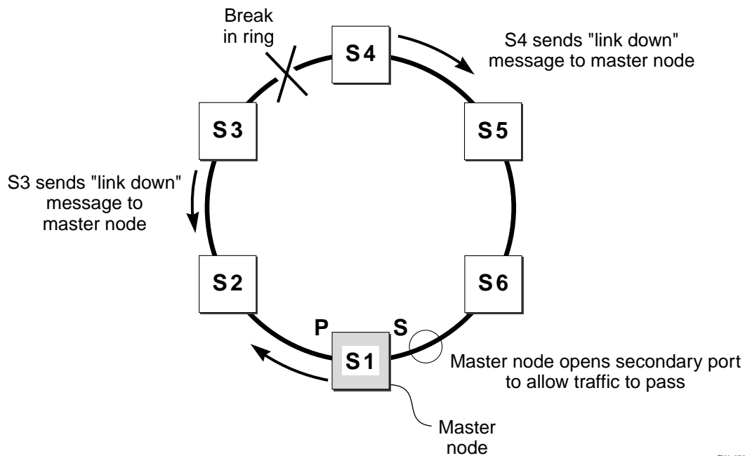
Figure 34: EAPS fault detection and protection switching
