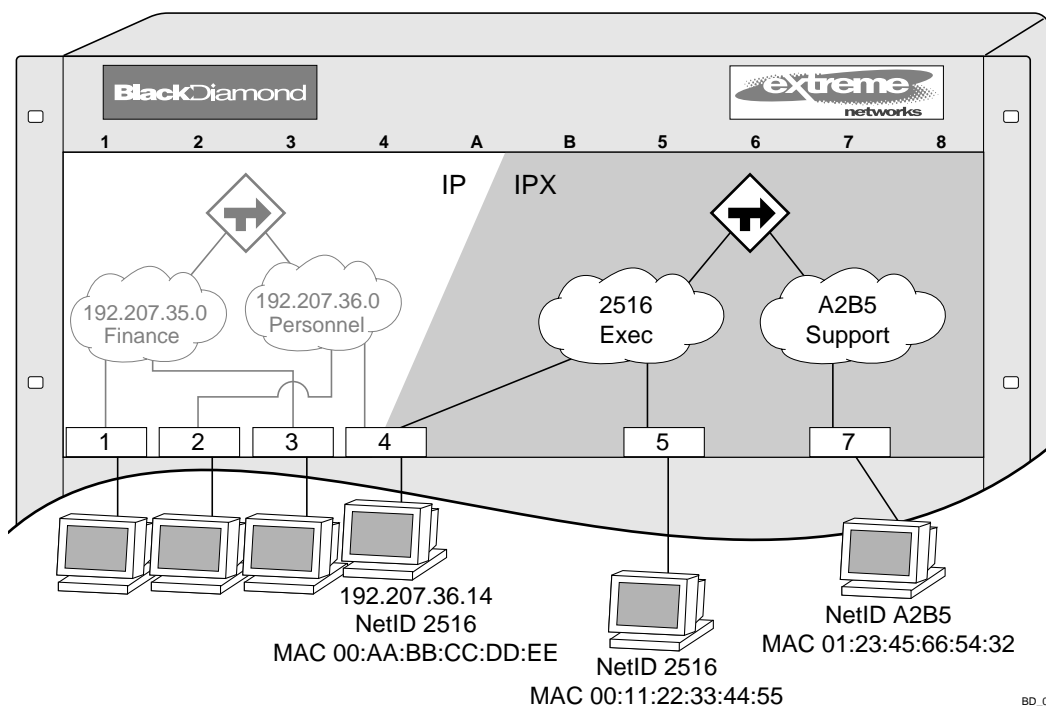
Figure 72: IPX routing configuration example
