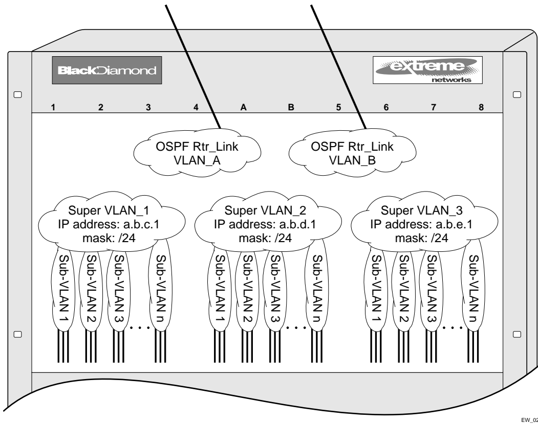
Figure 61: VLAN aggregation
