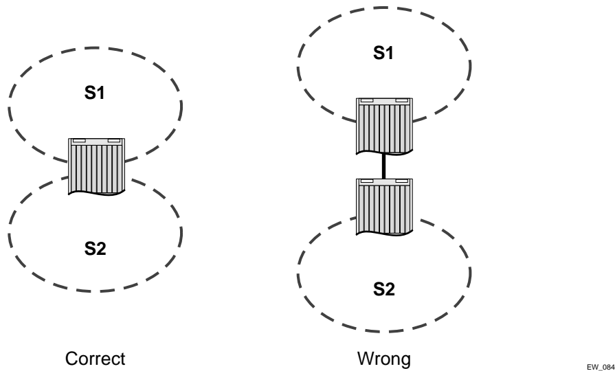
Figure 42: VLANs traverse domains inside switches
