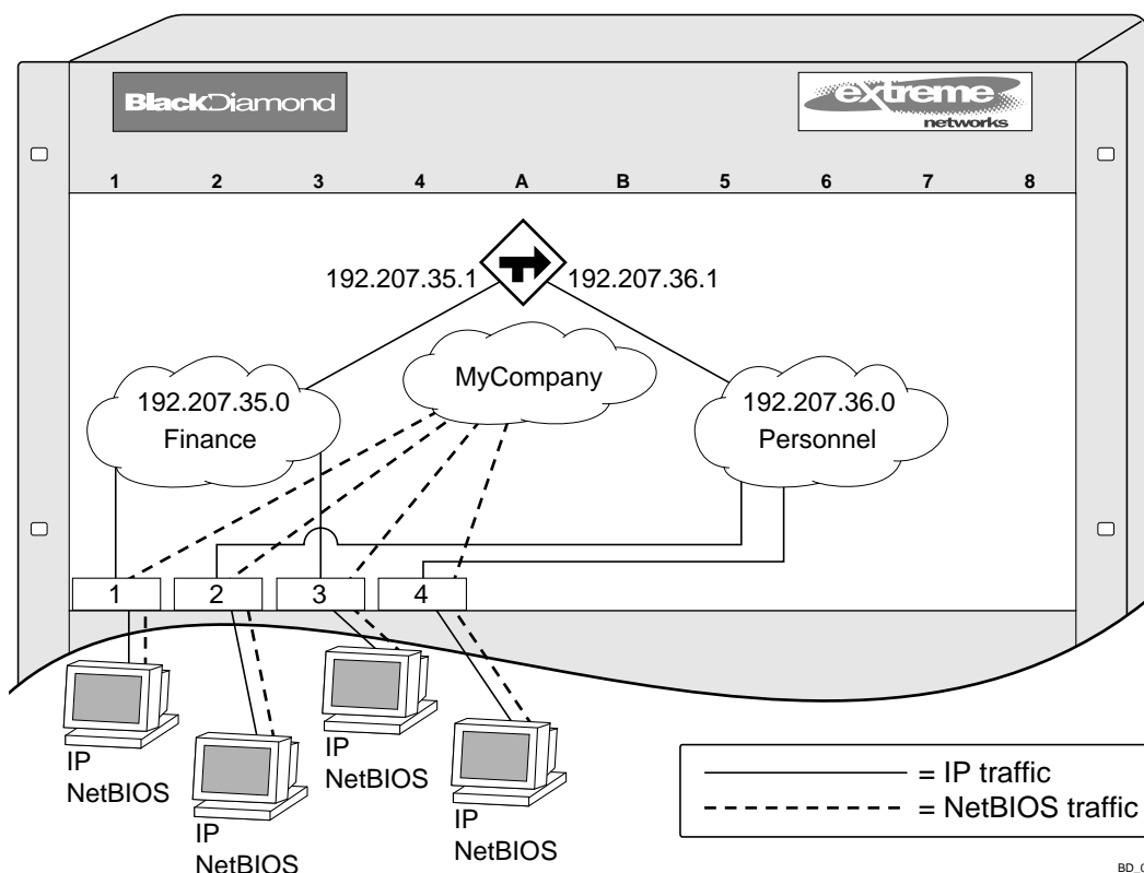
Figure 65: RIP configuration example
