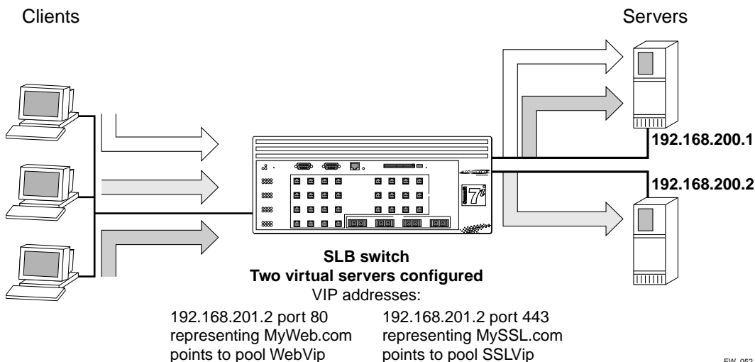
Figure 25: Transparent mode
