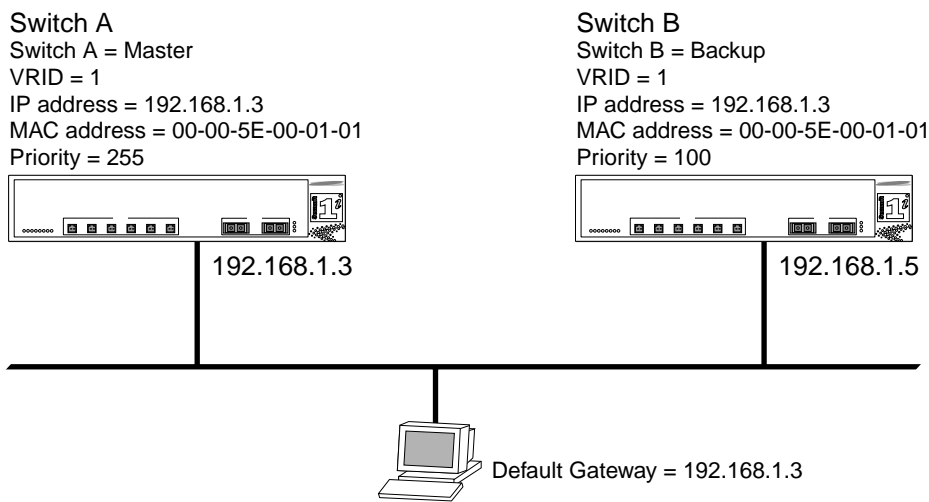
Figure 57: Simple VRRP network
