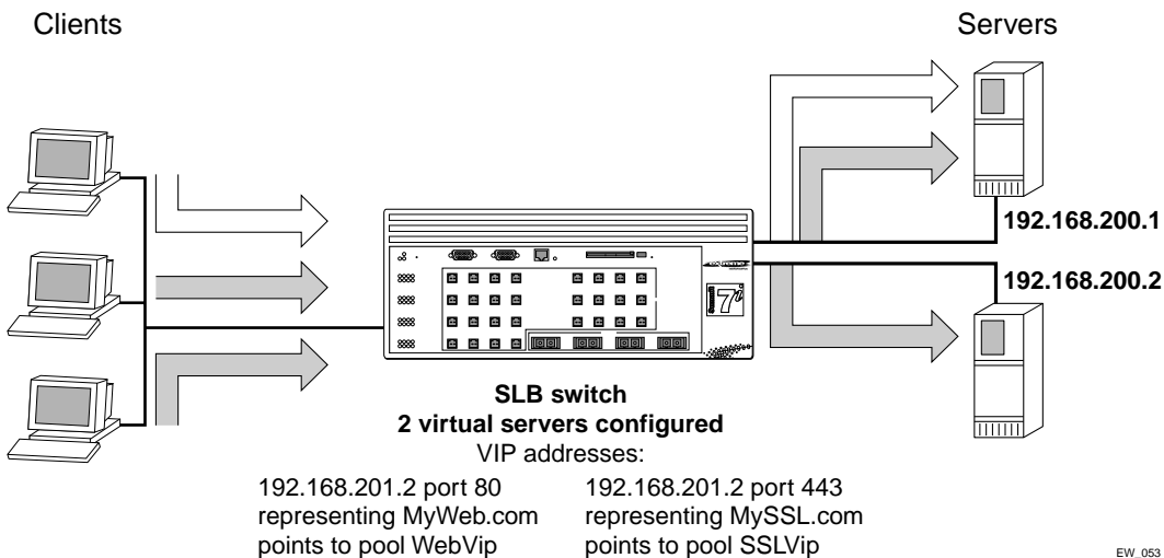
Figure 26: translation mode
