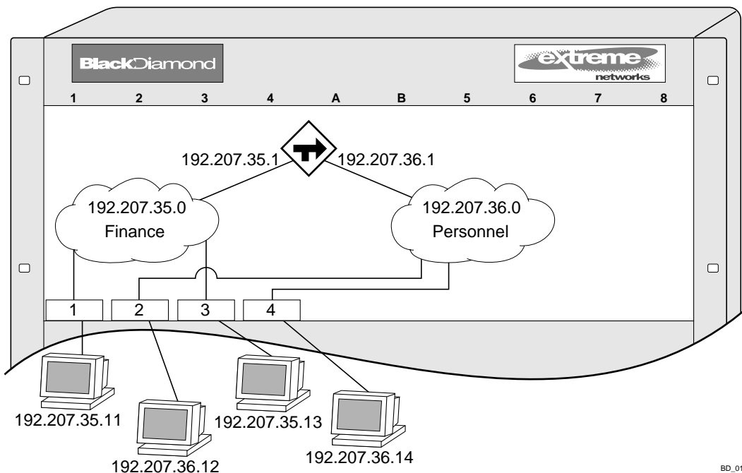
Figure 59: Routing between VLANs
