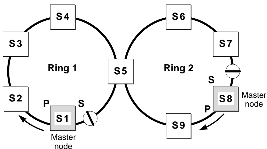
Figure 35: EAPS data VLAN spanning two rings interconnected by one switch
