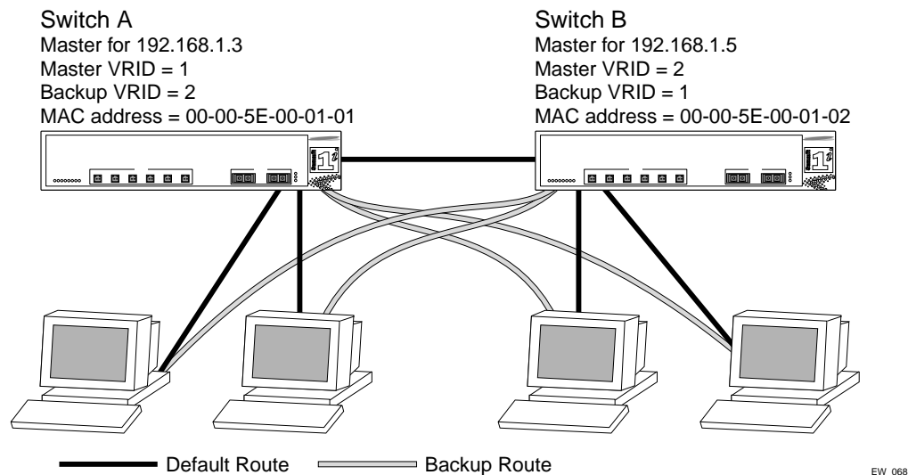
Figure 58: Fully-redundant VRRP configuration
