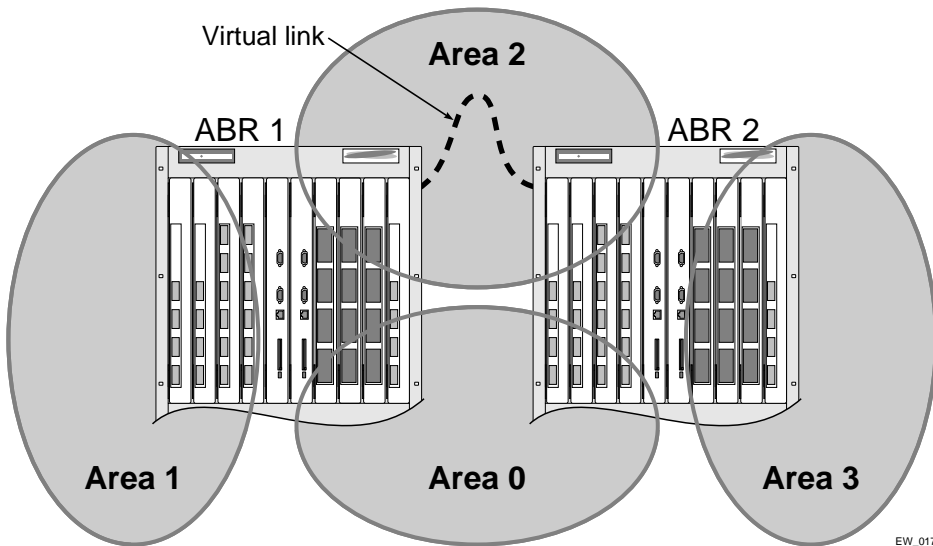
Figure 63: Virtual link providing redundancy
