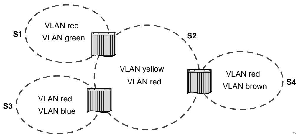
Figure 44: EMISTP configuration example
