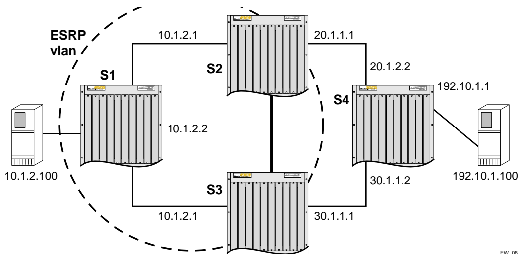
Figure 10: MAC address limits and ESRP-enabled VLANs
