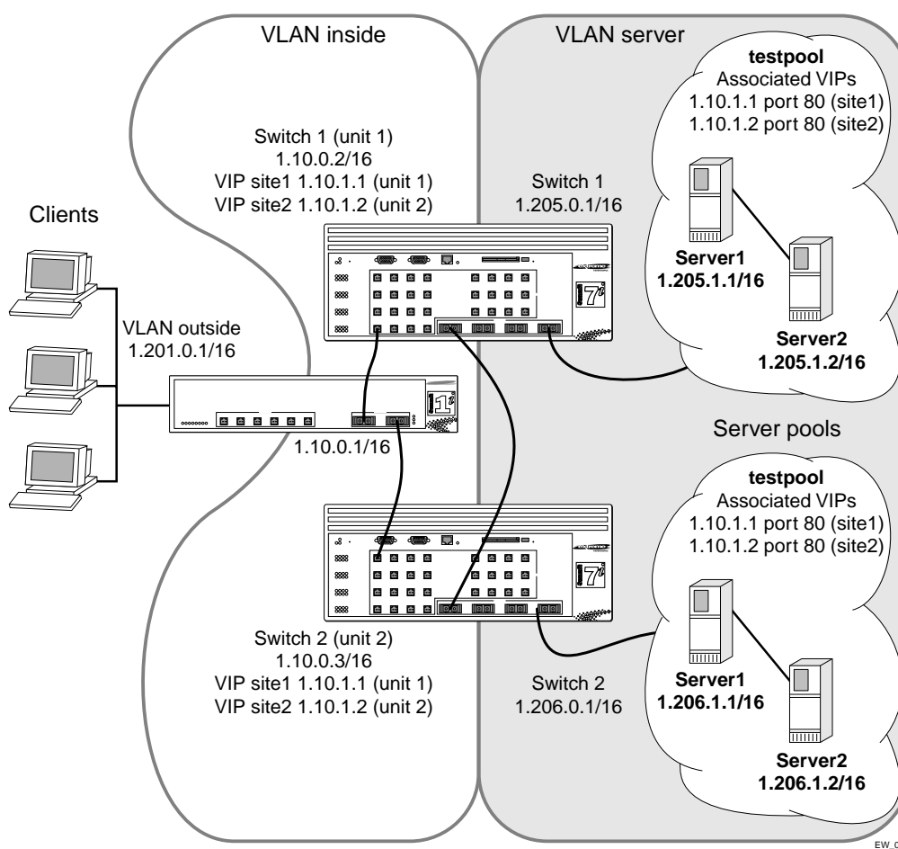
Figure 30: Active-active configuration
