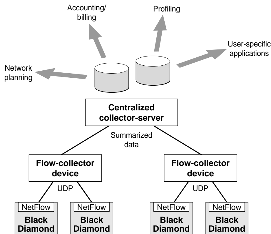
Figure 37: NetFlow Collection Architecture Example
