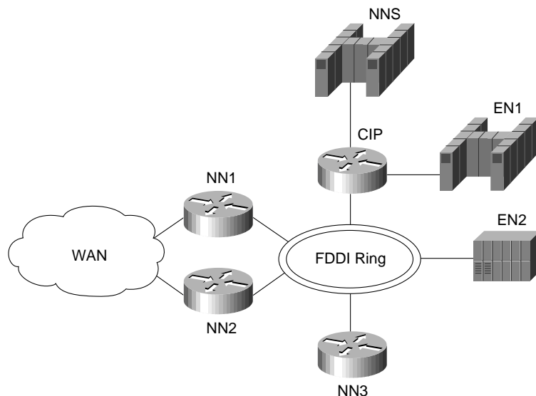
Figure 6-6 Physical view of an APPN network.
